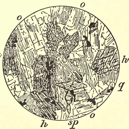
Fig. 26.—Syenite. Plauenscher Grund, Dresden. \times 8 . h , Green hornblende. o , Orthoclase, fairly prismatic in habit. q , Accessory interstitial quartz. sp , Sphene, marked out by its high refractive index and lozenge-shaped sections.
